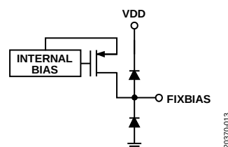
Figure 14. FIXBIAS Interface Schematic (Input)
