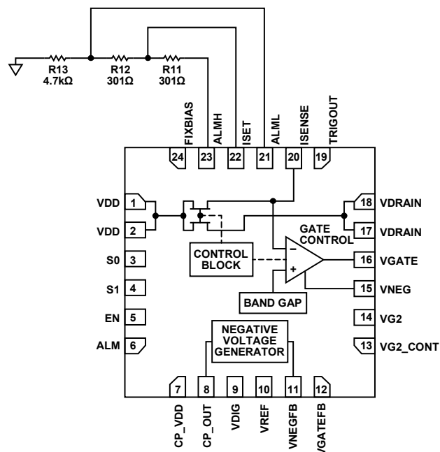
Figure 37. Current Alarm Resistor Configuration for \pm 6\% Thresholds
