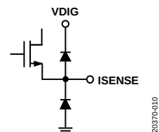
Figure 11. ISENSE Interface Schematic (Input)
