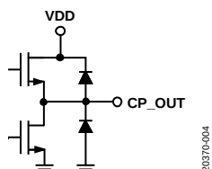
Figure 5. CP_OUT Interface Schematic (Output)
