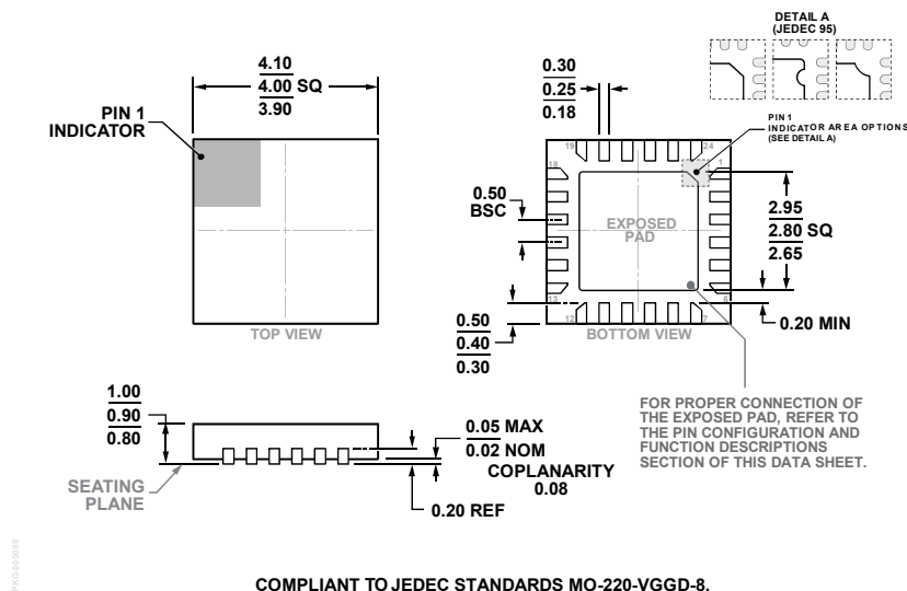
Figure 49. 24-Lead Lead Frame Chip Scale Package [LFCSP] 4 mm × 4 mm Body and 0.90 mm Package Height (HCP-24-2)
