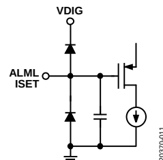
Figure 12. ALML, ISET Interface Schematic (Input)
