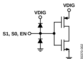
Figure 3. S1, S0, and EN Interface Schematic (Input)
