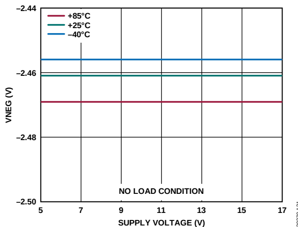
Figure 31. VNEG vs. Supply Voltage
